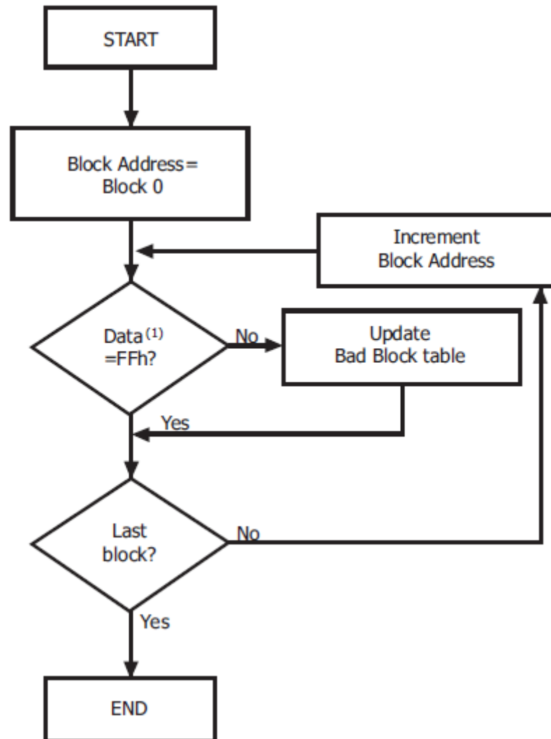
Figure 28 : Bad Block Management Flowchart
